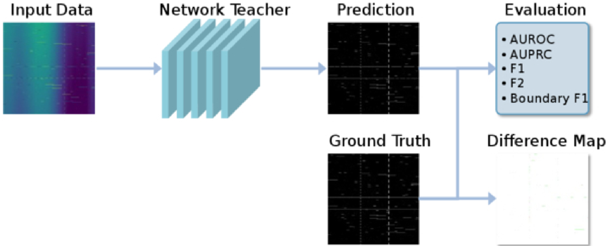
Figure 2. from Suxun Zhu et al 2026 Astrophys. J. Suppl. 284 doi:10.3847/1538-4365/ae5d39 https://dx.doi.org/10.3847/1538-4365/ae5d39 © 2026. The Author(s). Published by the American Astronomical Society.
