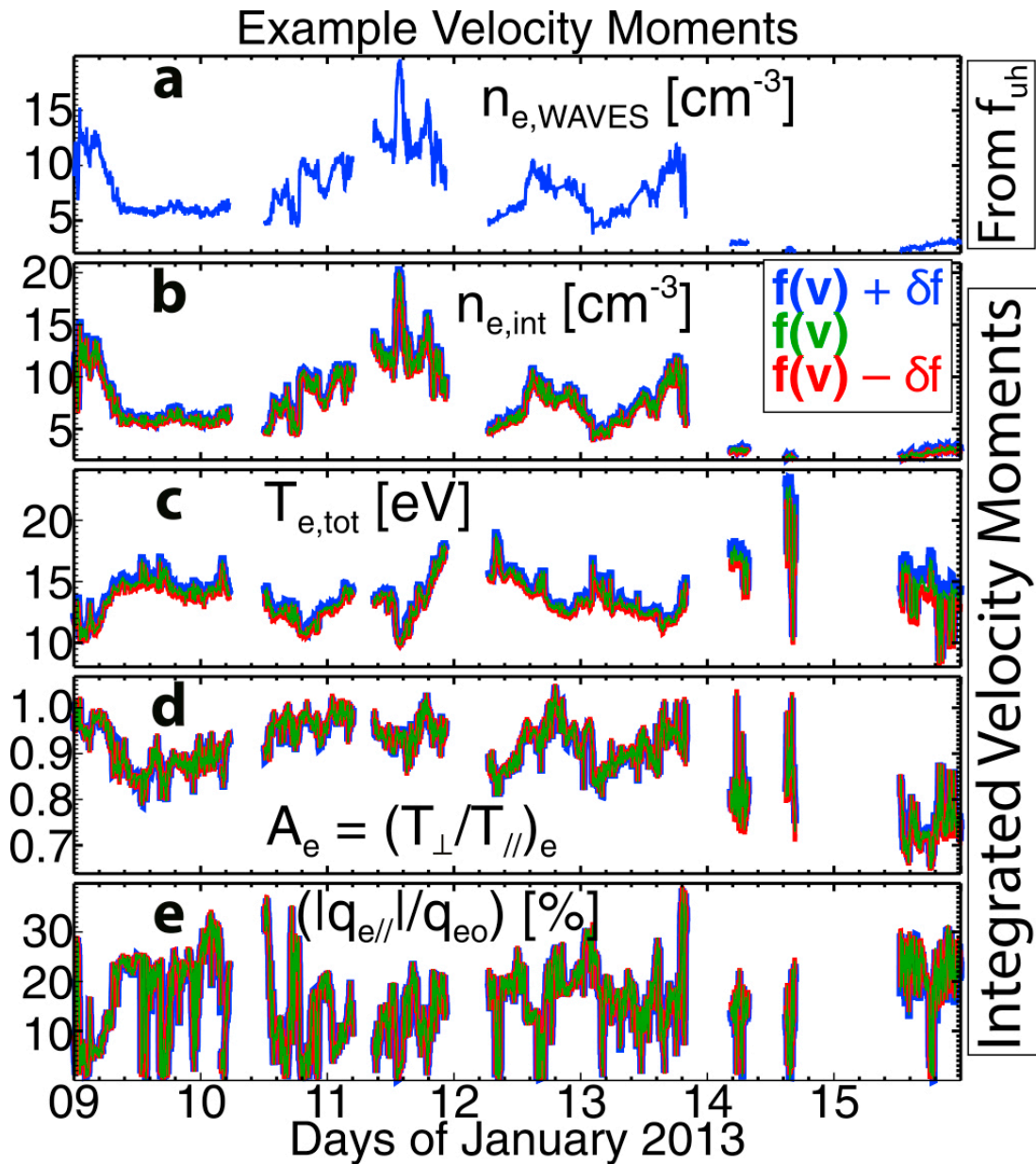
Figure 3. from Lynn B. Wilson et al 2026 Astrophys. J. Suppl. 284 doi:10.3847/1538-4365/ae5d2f https://dx.doi.org/10.3847/1538-4365/ae5d2f © 2026. The Author(s). Published by the American Astronomical Society.
