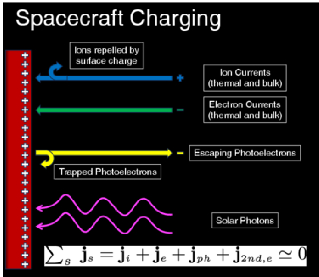
Figure 1. from Lynn B. Wilson et al 2026 Astrophys. J. Suppl. 284 doi:10.3847/1538-4365/ae5d2f https://dx.doi.org/10.3847/1538-4365/ae5d2f © 2026. The Author(s). Published by the American Astronomical Society.
