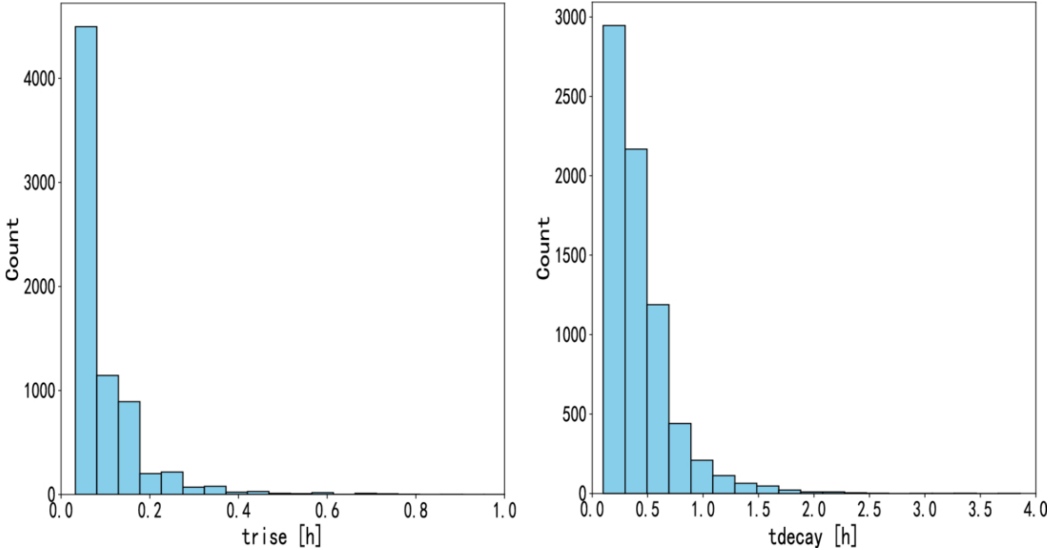
Figure 2. from Lulu Xu et al 2026 Astrophys. J. Suppl. 284 doi:10.3847/1538-4365/ae5d2d https://dx.doi.org/10.3847/1538-4365/ae5d2d © 2026. The Author(s). Published by the American Astronomical Society.
