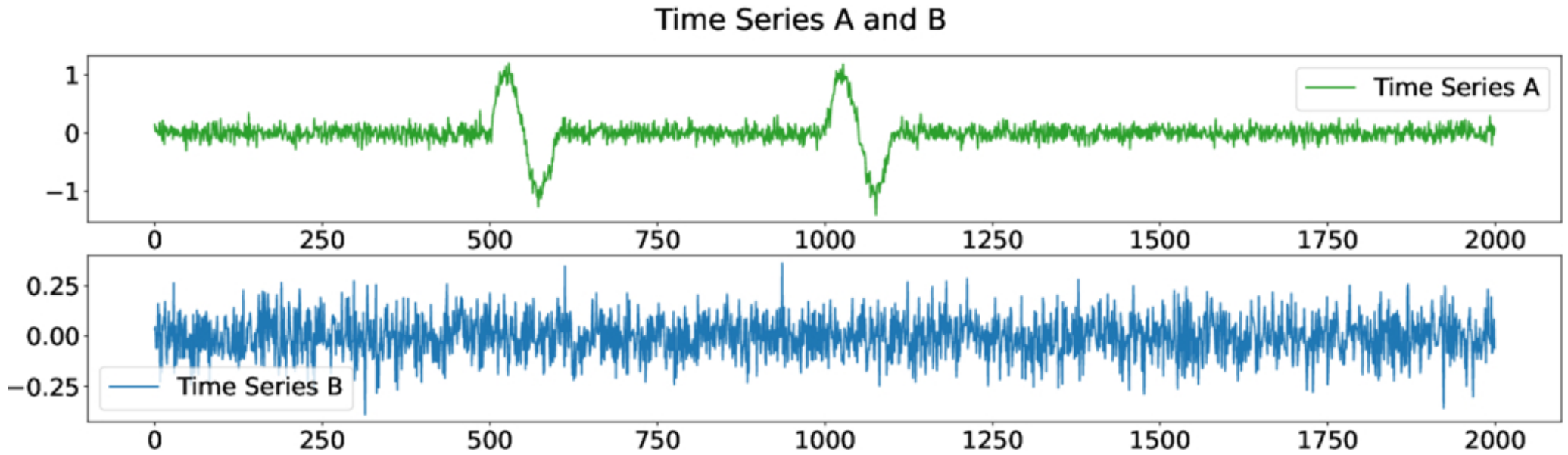
Figure 4. from Drew Watson et al 2026 Astrophys. J. Suppl. 284 doi:10.3847/1538-4365/ae5c04 https://dx.doi.org/10.3847/1538-4365/ae5c04 © 2026. The Author(s). Published by the American Astronomical Society.
