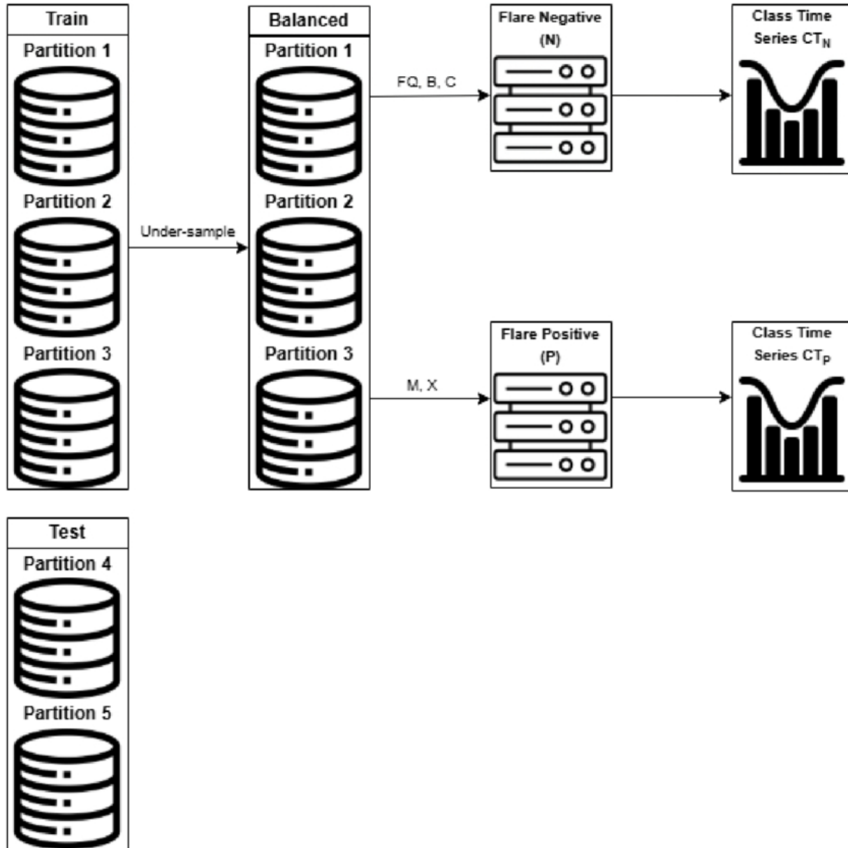
Figure 3. from Drew Watson et al 2026 Astrophys. J. Suppl. 284 doi:10.3847/1538-4365/ae5c04 https://dx.doi.org/10.3847/1538-4365/ae5c04 © 2026. The Author(s). Published by the American Astronomical Society.
