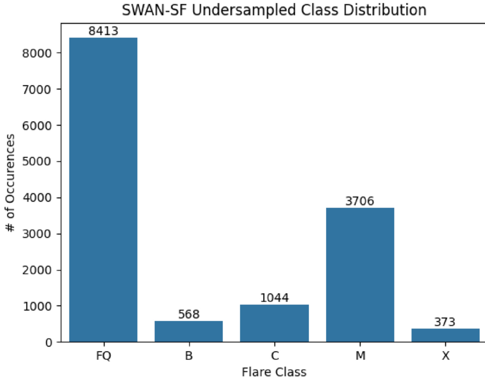
Figure 2. from Drew Watson et al 2026 Astrophys. J. Suppl. 284 doi:10.3847/1538-4365/ae5c04 https://dx.doi.org/10.3847/1538-4365/ae5c04 © 2026. The Author(s). Published by the American Astronomical Society.
