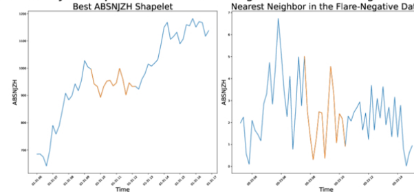
Best ABSNJZH Shapelet and its Nearest Neighbor in the Flare-Negative Data
