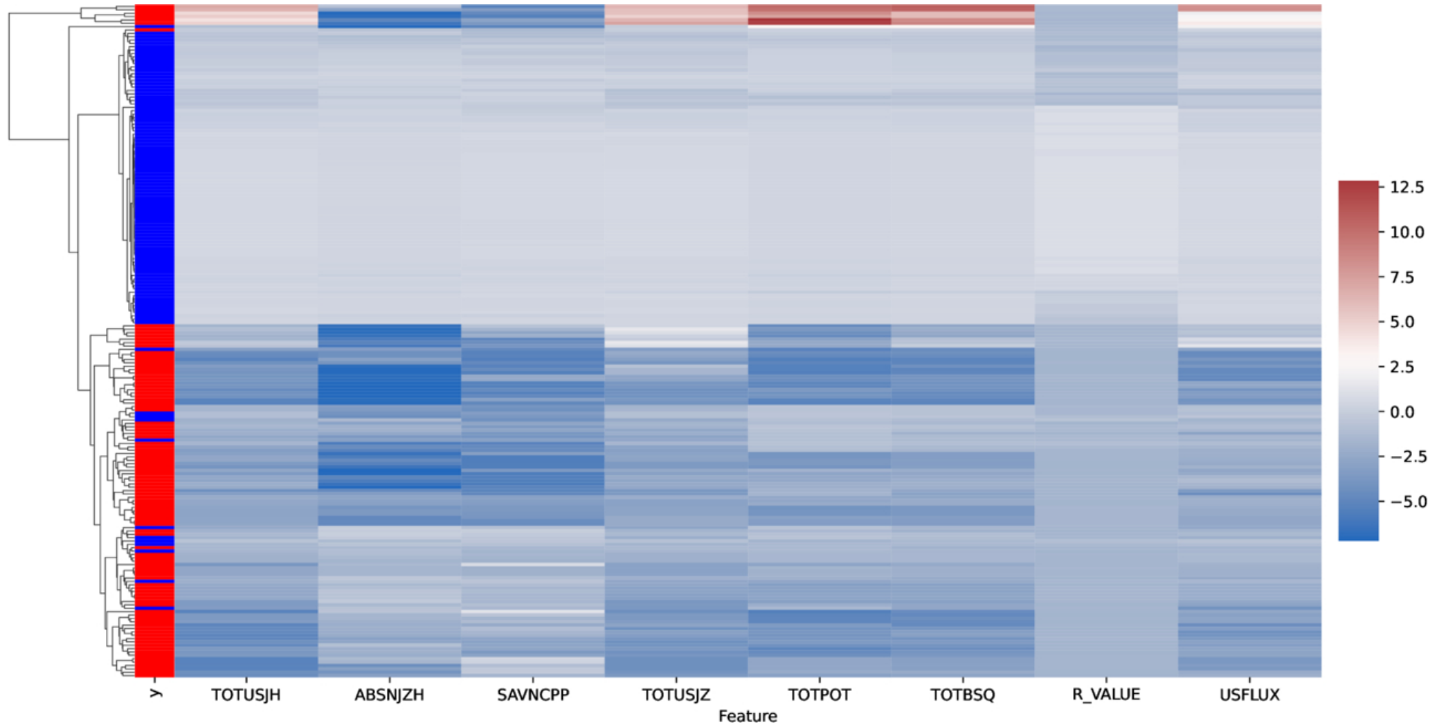
Figure 13. from Drew Watson et al 2026 Astrophys. J. Suppl. 284 doi:10.3847/1538-4365/ae5c04 https://dx.doi.org/10.3847/1538-4365/ae5c04 © 2026. The Author(s). Published by the American Astronomical Society.
