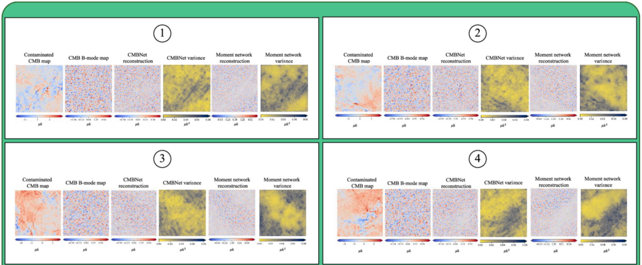
Figure 2. from Ma Long et al 2026 Astrophys. J. Suppl. 284 doi:10.3847/1538-4365/ae5c01 https://dx.doi.org/10.3847/1538-4365/ae5c01 © 2026. The Author(s). Published by the American Astronomical Society.
