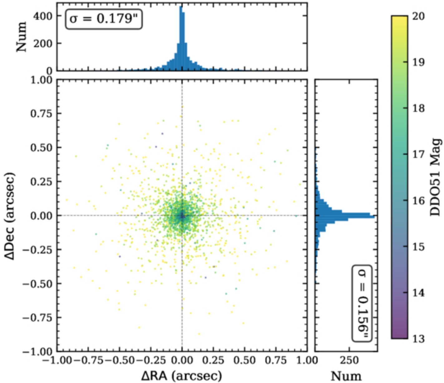
Figure 5. from Qiqian Zhang et al 2026 Astrophys. J. Suppl. 284 doi:10.3847/1538-4365/ae5b7e https://dx.doi.org/10.3847/1538-4365/ae5b7e © 2026. The Author(s). Published by the American Astronomical Society.
