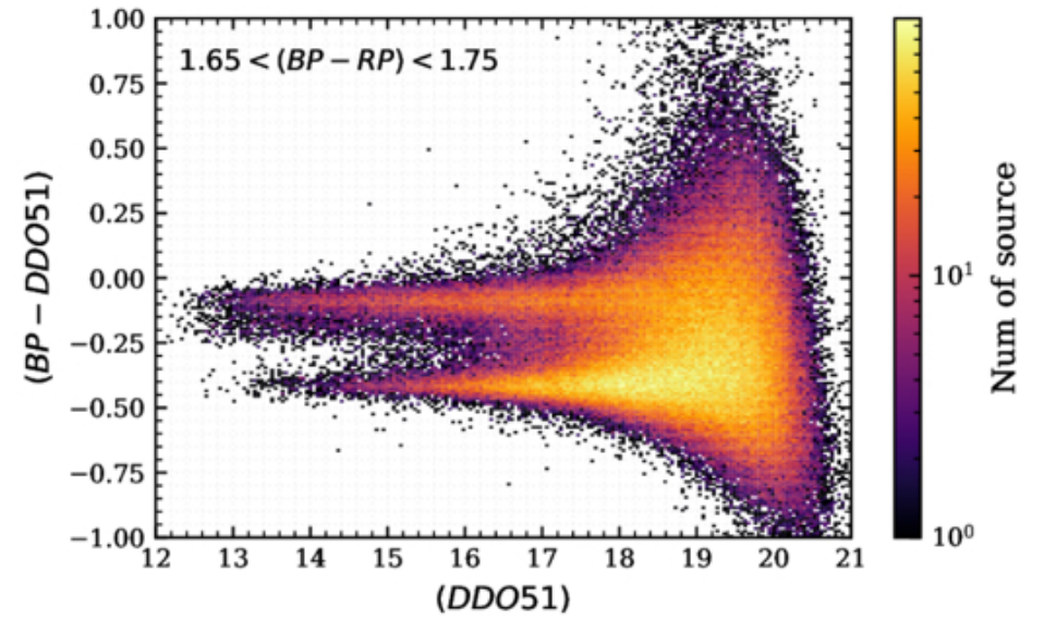
(b) Color-Magnitude Diagram
