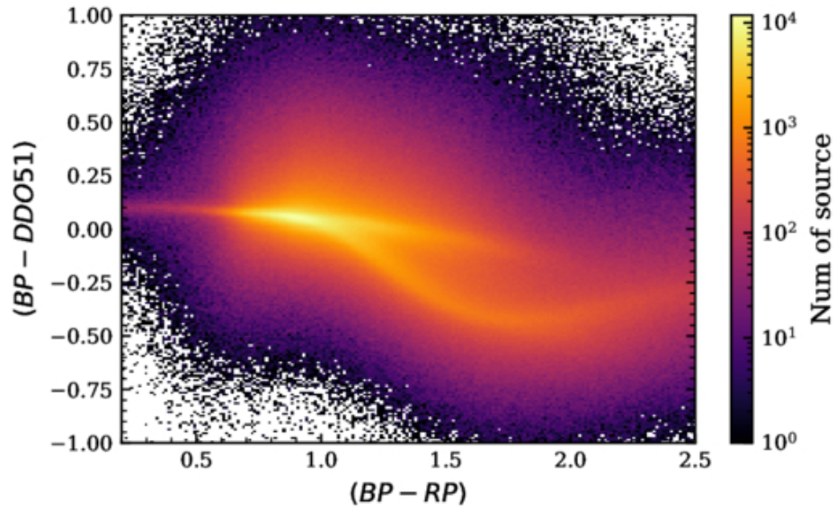
(a) Color-Color Diagram
