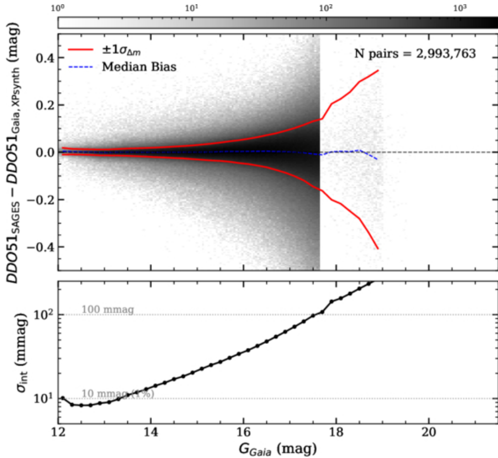
(a) SAGES v.s. Gaia XPS
