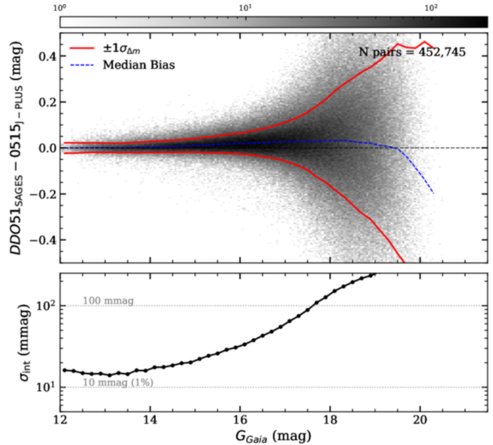
(b) SAGES v.s. J-PLUS
