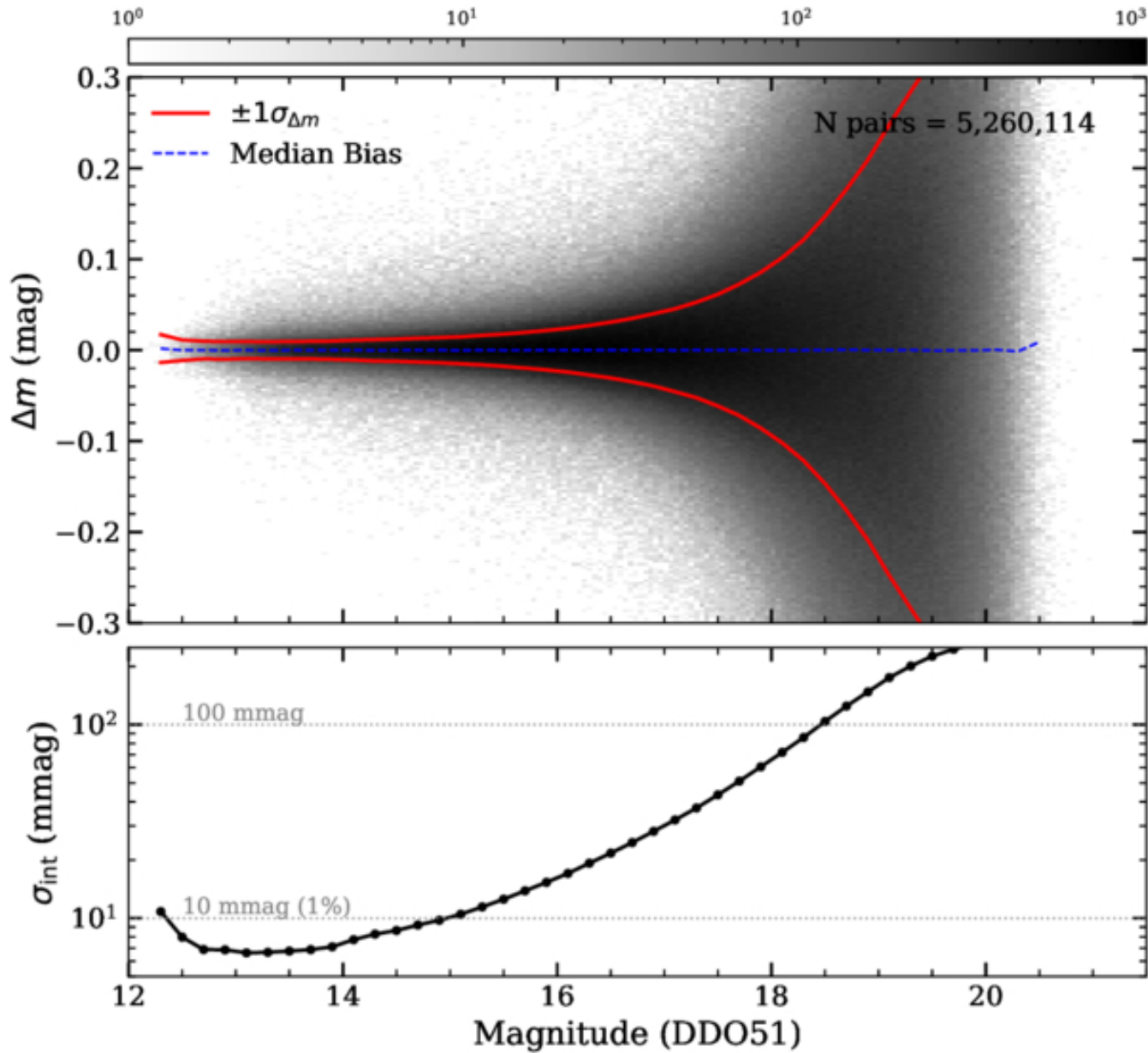
Figure 12. from Qiqian Zhang et al 2026 Astrophys. J. Suppl. 284 doi:10.3847/1538-4365/ae5b7e https://dx.doi.org/10.3847/1538-4365/ae5b7e © 2026. The Author(s). Published by the American Astronomical Society.
