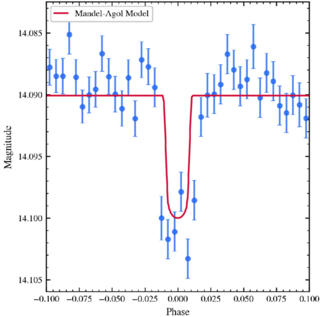
Figure 7. from Joshua T. Roth et al 2026 Astrophys. J. Suppl. 284 doi:10.3847/1538-4365/ae5b6c https://dx.doi.org/10.3847/1538-4365/ae5b6c © 2026. The Author(s). Published by the American Astronomical Society.
