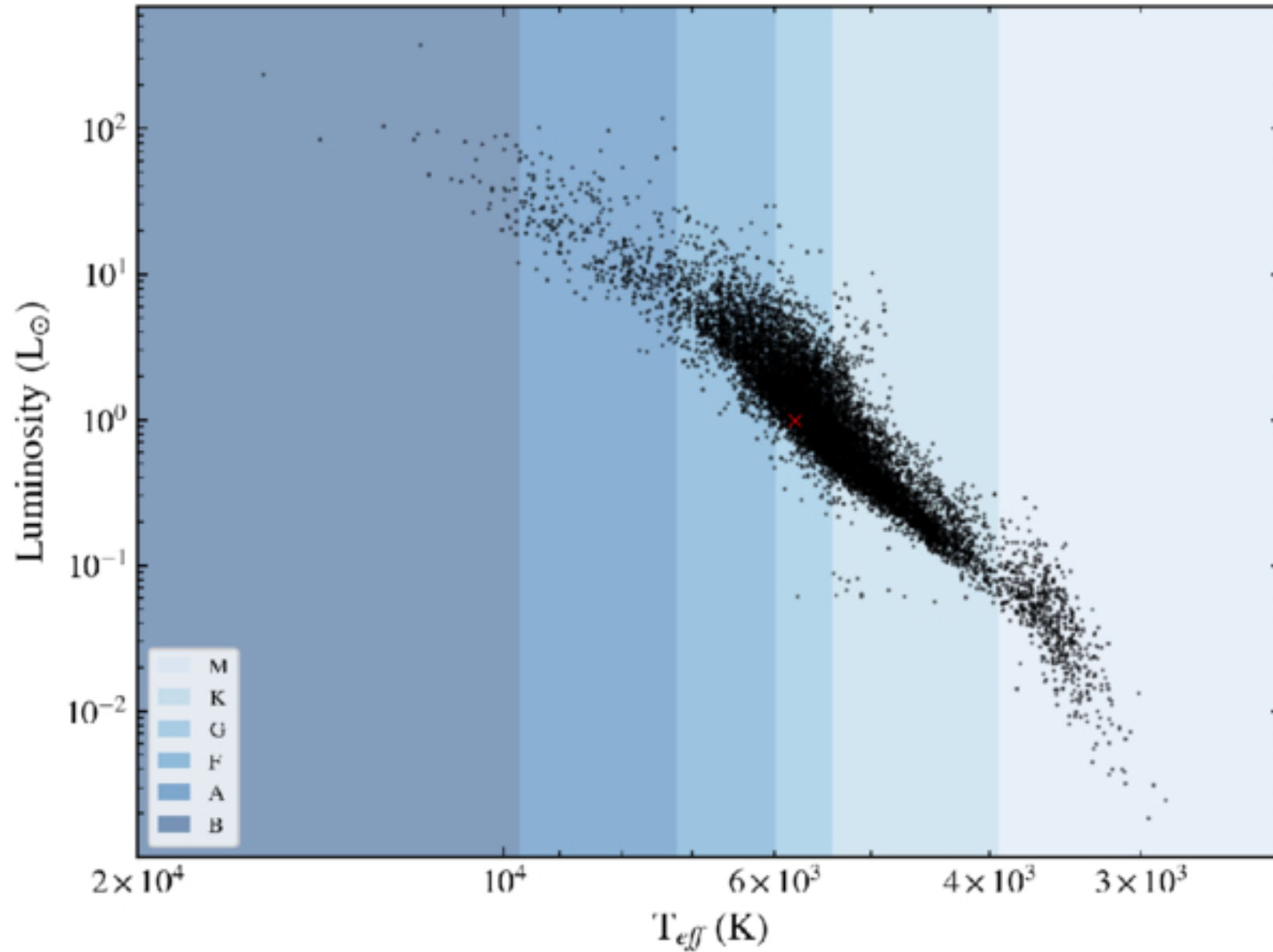
Figure 12. from Joshua T. Roth et al 2026 Astrophys. J. Suppl. 284 doi:10.3847/1538-4365/ae5b6c https://dx.doi.org/10.3847/1538-4365/ae5b6c © 2026. The Author(s). Published by the American Astronomical Society.
