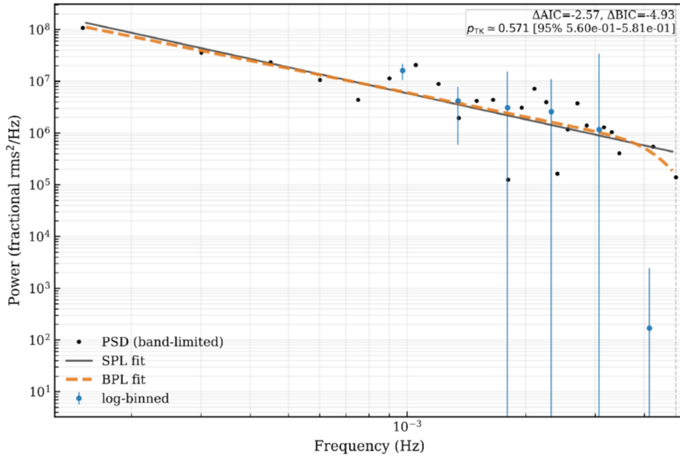
Figure 2. from S.-Y. Wu et al 2026 Astrophys. J. Suppl. 284 doi:10.3847/1538-4365/ae5a2c https://dx.doi.org/10.3847/1538-4365/ae5a2c © 2026. The Author(s). Published by the American Astronomical Society.
