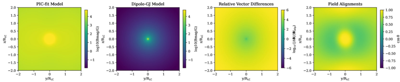
PSR J1856-3754 | View along Y-axis: B_y
