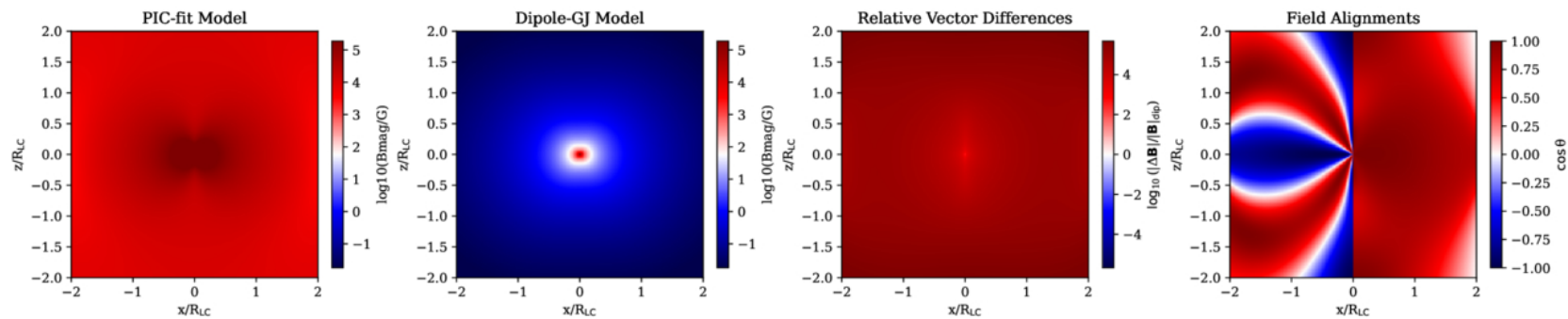
PSR J1856-3754 | View along Z-axis: B_z
