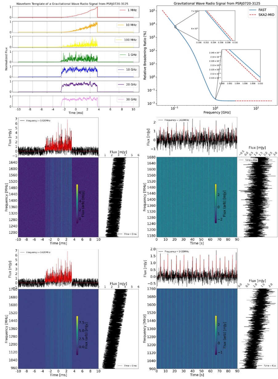
Figure 4. from Wei Hong et al 2026 Astrophys. J. Suppl. 284 doi:10.3847/1538-4365/ae593d https://dx.doi.org/10.3847/1538-4365/ae593d © 2026. The Author(s). Published by the American Astronomical Society.
