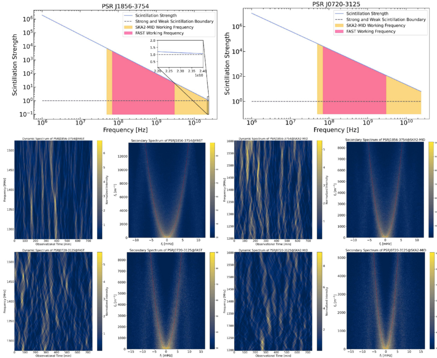
Figure 14. from Wei Hong et al 2026 Astrophys. J. Suppl. 284 doi:10.3847/1538-4365/ae593d https://dx.doi.org/10.3847/1538-4365/ae593d © 2026. The Author(s). Published by the American Astronomical Society.
