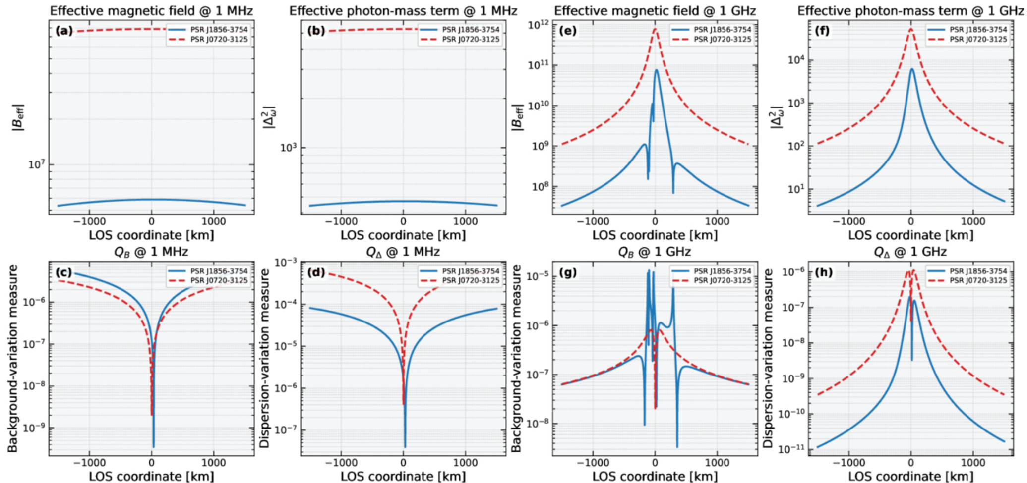
Figure 12. from Wei Hong et al 2026 Astrophys. J. Suppl. 284 doi:10.3847/1538-4365/ae593d https://dx.doi.org/10.3847/1538-4365/ae593d © 2026. The Author(s). Published by the American Astronomical Society.
