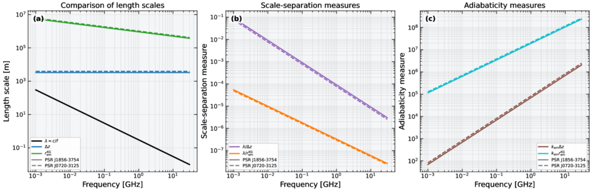
Figure 11. from Wei Hong et al 2026 Astrophys. J. Suppl. 284 doi:10.3847/1538-4365/ae593d https://dx.doi.org/10.3847/1538-4365/ae593d © 2026. The Author(s). Published by the American Astronomical Society.
