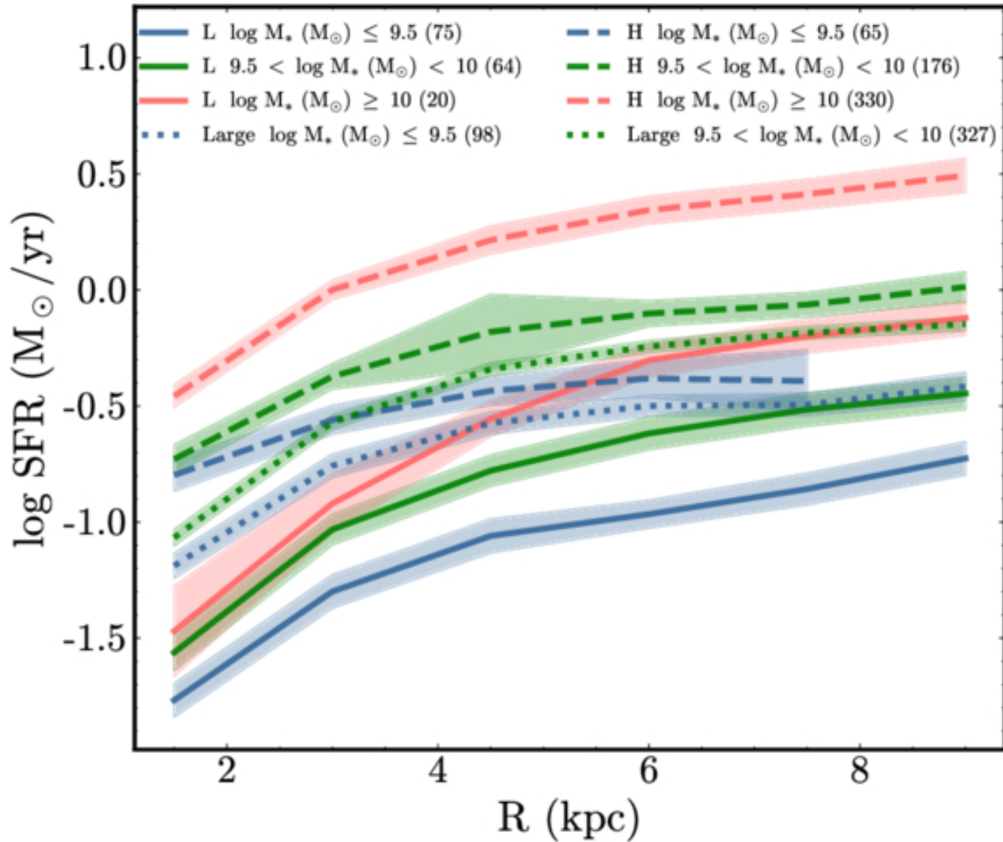
Figure 9. from Mengting Shen et al 2026 Astrophys. J. Suppl. 284 doi:10.3847/1538-4365/ae5929 https://dx.doi.org/10.3847/1538-4365/ae5929 © 2026. The Author(s). Published by the American Astronomical Society.
