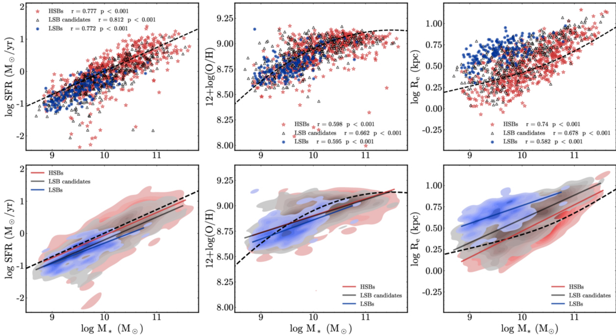
Figure 4. from Mengting Shen et al 2026 Astrophys. J. Suppl. 284 doi:10.3847/1538-4365/ae5929 https://dx.doi.org/10.3847/1538-4365/ae5929 © 2026. The Author(s). Published by the American Astronomical Society.
