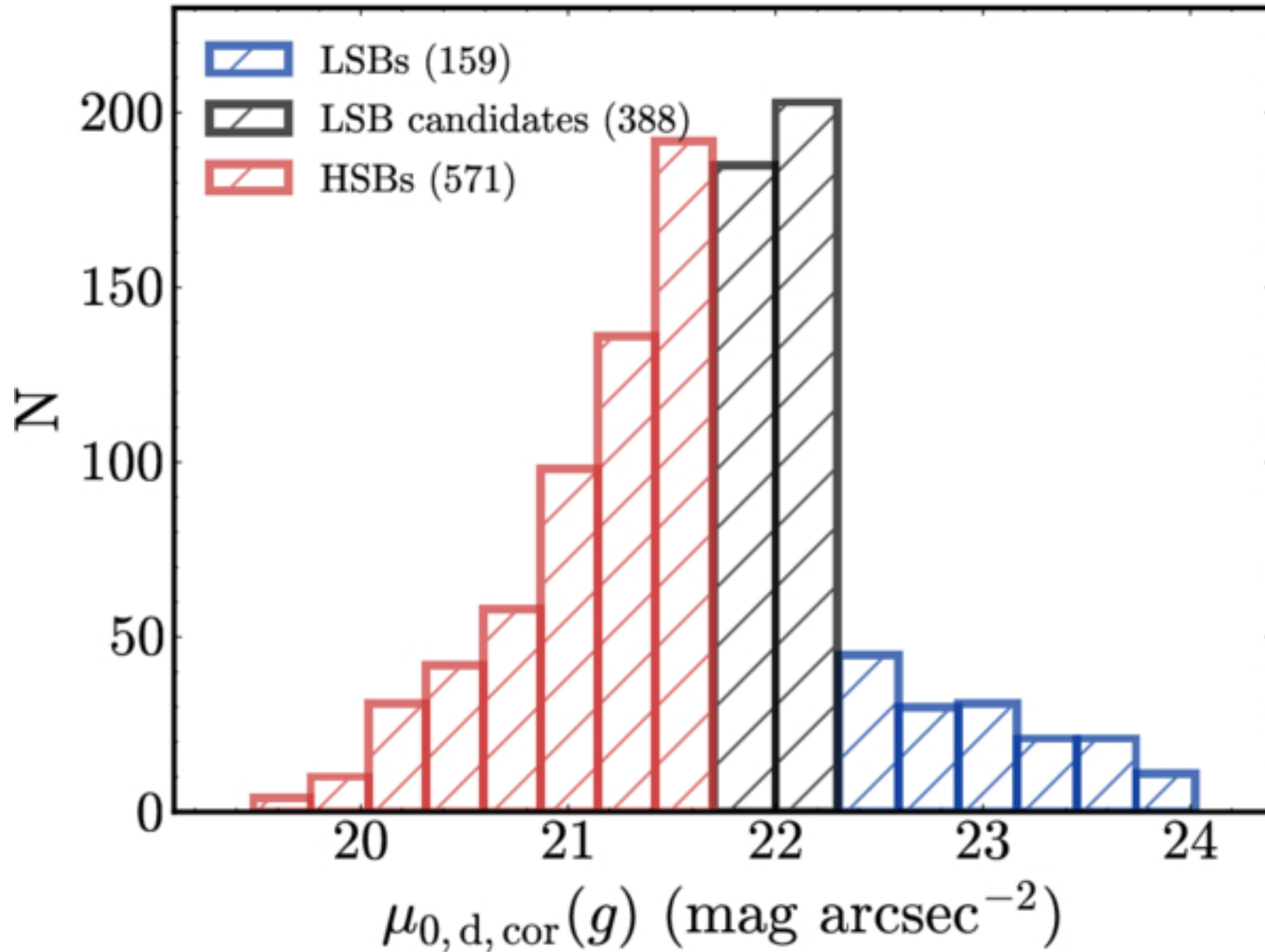
Figure 3. from Mengting Shen et al 2026 Astrophys. J. Suppl. 284 doi:10.3847/1538-4365/ae5929 https://dx.doi.org/10.3847/1538-4365/ae5929 © 2026. The Author(s). Published by the American Astronomical Society.
