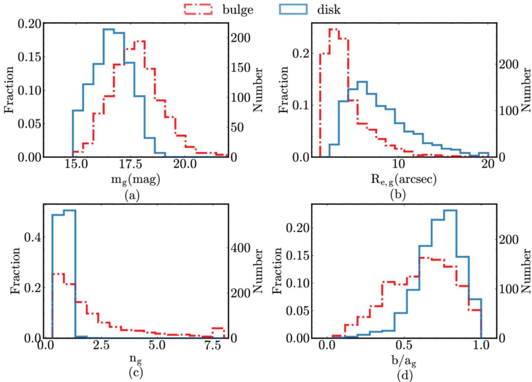
Figure 2. from Mengting Shen et al 2026 Astrophys. J. Suppl. 284 doi:10.3847/1538-4365/ae5929 https://dx.doi.org/10.3847/1538-4365/ae5929 © 2026. The Author(s). Published by the American Astronomical Society.
