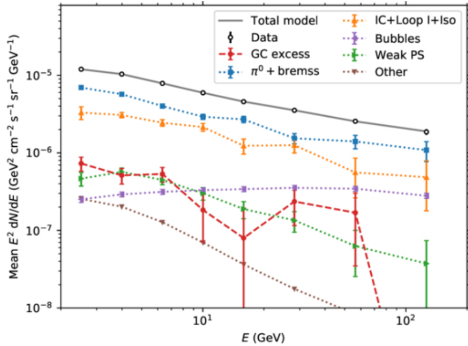
Figure 8. from F. Alemanno et al 2026 Astrophys. J. Suppl. 284 doi:10.3847/1538-4365/ae58a1 https://dx.doi.org/10.3847/1538-4365/ae58a1 © 2026. The Author(s). Published by the American Astronomical Society.
