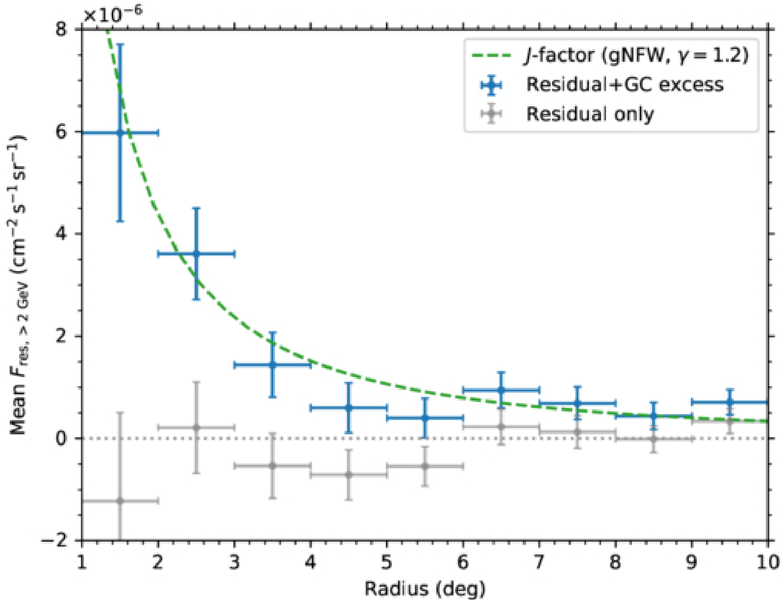
Figure 7. from F. Alemanno et al 2026 Astrophys. J. Suppl. 284 doi:10.3847/1538-4365/ae58a1 https://dx.doi.org/10.3847/1538-4365/ae58a1 © 2026. The Author(s). Published by the American Astronomical Society.
