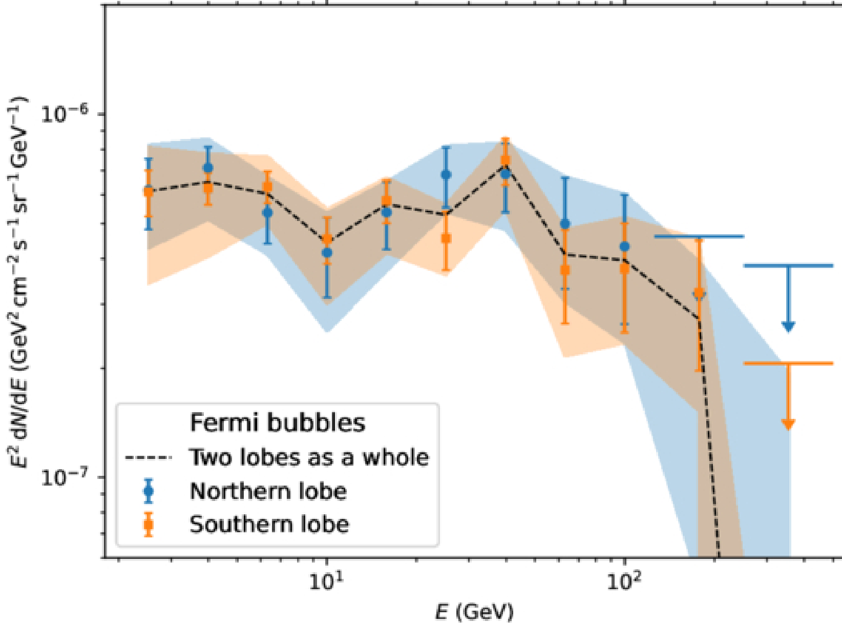
Figure 5. from F. Alemanno et al 2026 Astrophys. J. Suppl. 284 doi:10.3847/1538-4365/ae58a1 https://dx.doi.org/10.3847/1538-4365/ae58a1 © 2026. The Author(s). Published by the American Astronomical Society.
