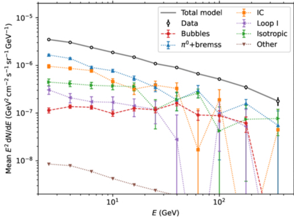
Figure 4. from F. Alemanno et al 2026 Astrophys. J. Suppl. 284 doi:10.3847/1538-4365/ae58a1 https://dx.doi.org/10.3847/1538-4365/ae58a1 © 2026. The Author(s). Published by the American Astronomical Society.
