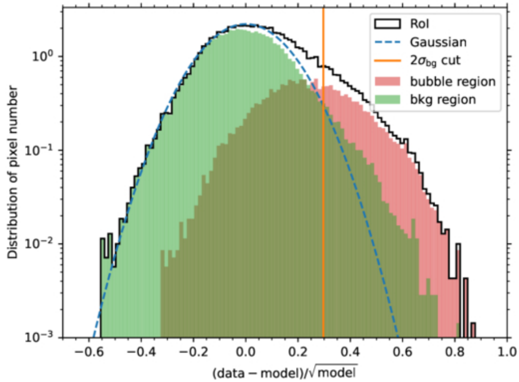
Figure 2. from F. Alemanno et al 2026 Astrophys. J. Suppl. 284 doi:10.3847/1538-4365/ae58a1 https://dx.doi.org/10.3847/1538-4365/ae58a1 © 2026. The Author(s). Published by the American Astronomical Society.
