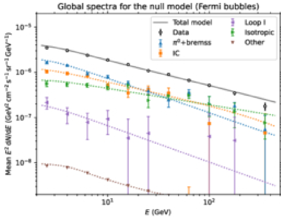
Figure 17. from F. Alemanno et al 2026 Astrophys. J. Suppl. 284 doi:10.3847/1538-4365/ae58a1 https://dx.doi.org/10.3847/1538-4365/ae58a1 © 2026. The Author(s). Published by the American Astronomical Society.
