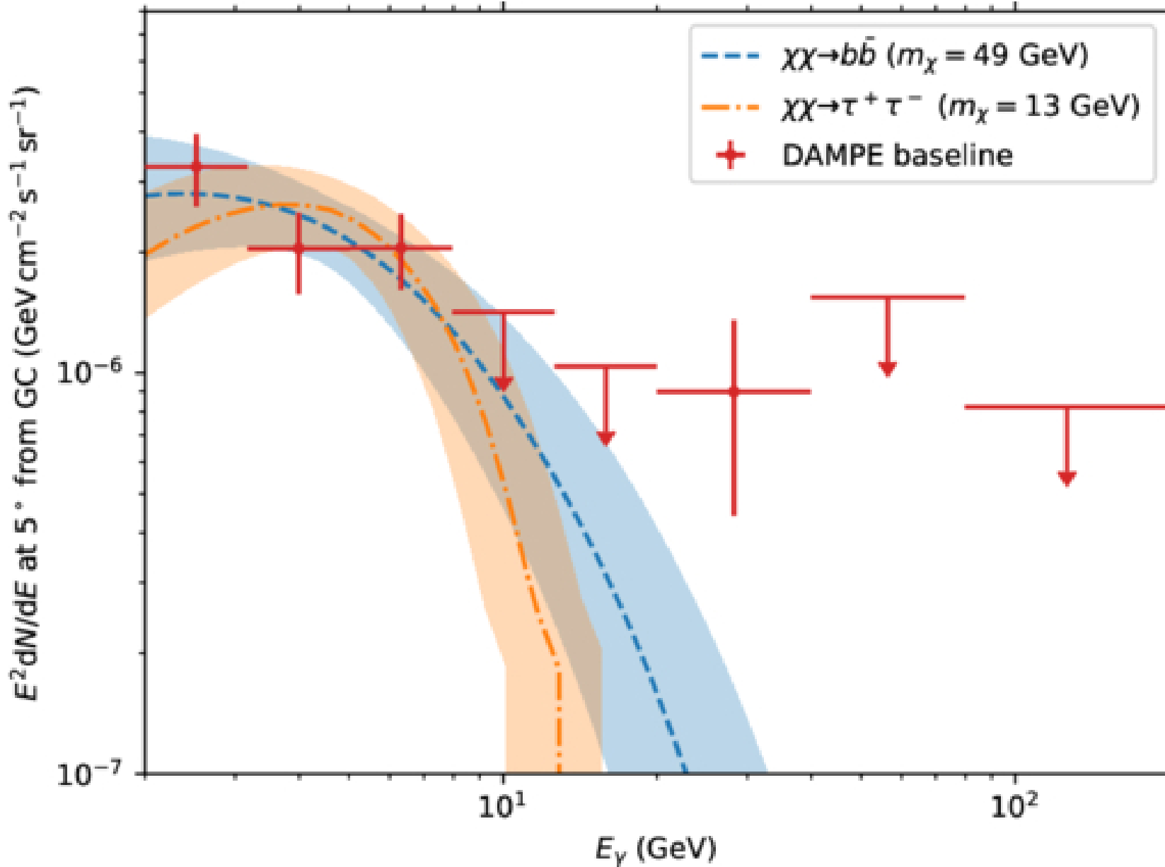
Figure 13. from F. Alemanno et al 2026 Astrophys. J. Suppl. 284 doi:10.3847/1538-4365/ae58a1 https://dx.doi.org/10.3847/1538-4365/ae58a1 © 2026. The Author(s). Published by the American Astronomical Society.
