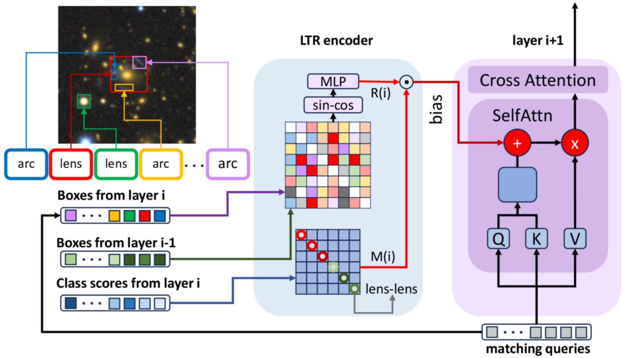
Figure 7. from Junyu Meng et al 2026 Astrophys. J. Suppl. 284 doi:10.3847/1538-4365/ae5812 https://dx.doi.org/10.3847/1538-4365/ae5812 © 2026. The Author(s). Published by the American Astronomical Society.
