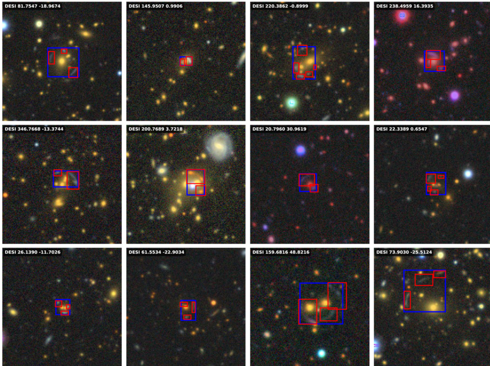
Figure 4. from Junyu Meng et al 2026 Astrophys. J. Suppl. 284 doi:10.3847/1538-4365/ae5812 https://dx.doi.org/10.3847/1538-4365/ae5812 © 2026. The Author(s). Published by the American Astronomical Society.
