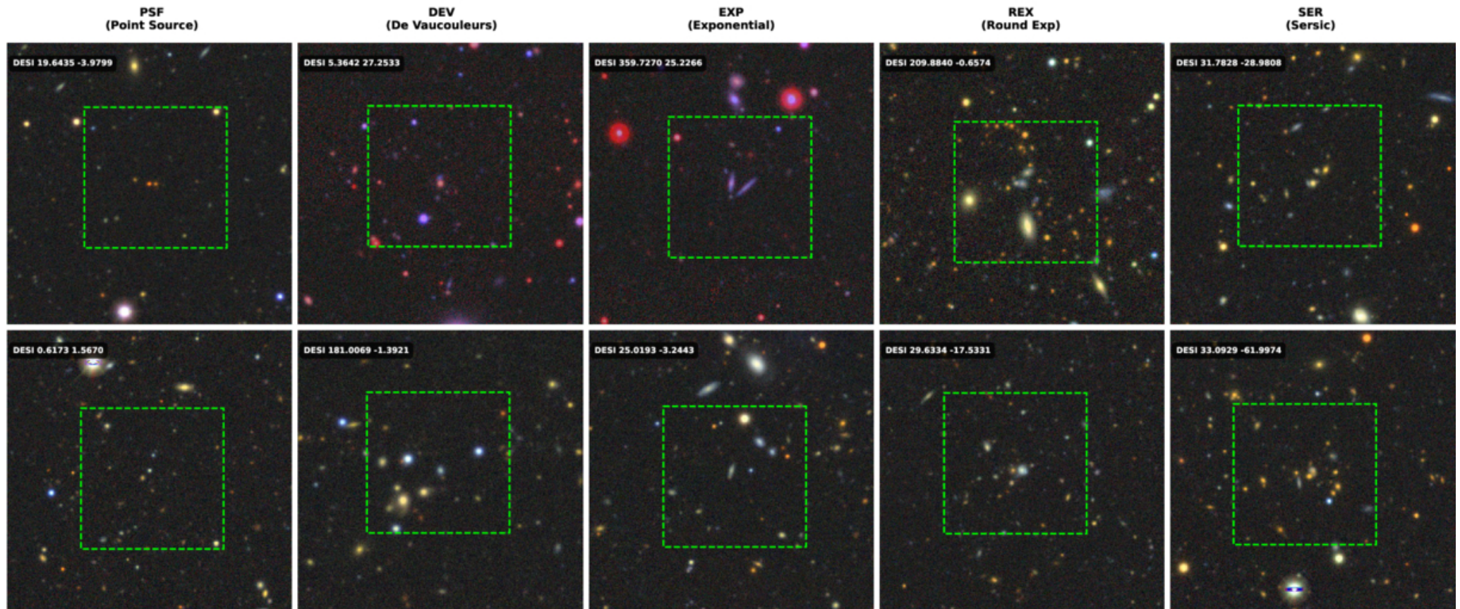
Figure 3. from Junyu Meng et al 2026 Astrophys. J. Suppl. 284 doi:10.3847/1538-4365/ae5812 https://dx.doi.org/10.3847/1538-4365/ae5812 © 2026. The Author(s). Published by the American Astronomical Society.
