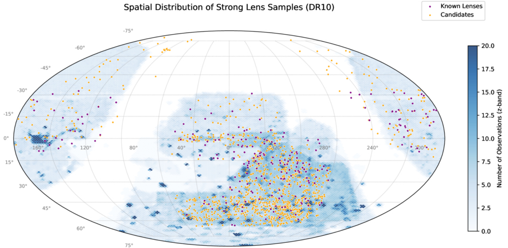
Figure 2. from Junyu Meng et al 2026 Astrophys. J. Suppl. 284 doi:10.3847/1538-4365/ae5812 https://dx.doi.org/10.3847/1538-4365/ae5812 © 2026. The Author(s). Published by the American Astronomical Society.
