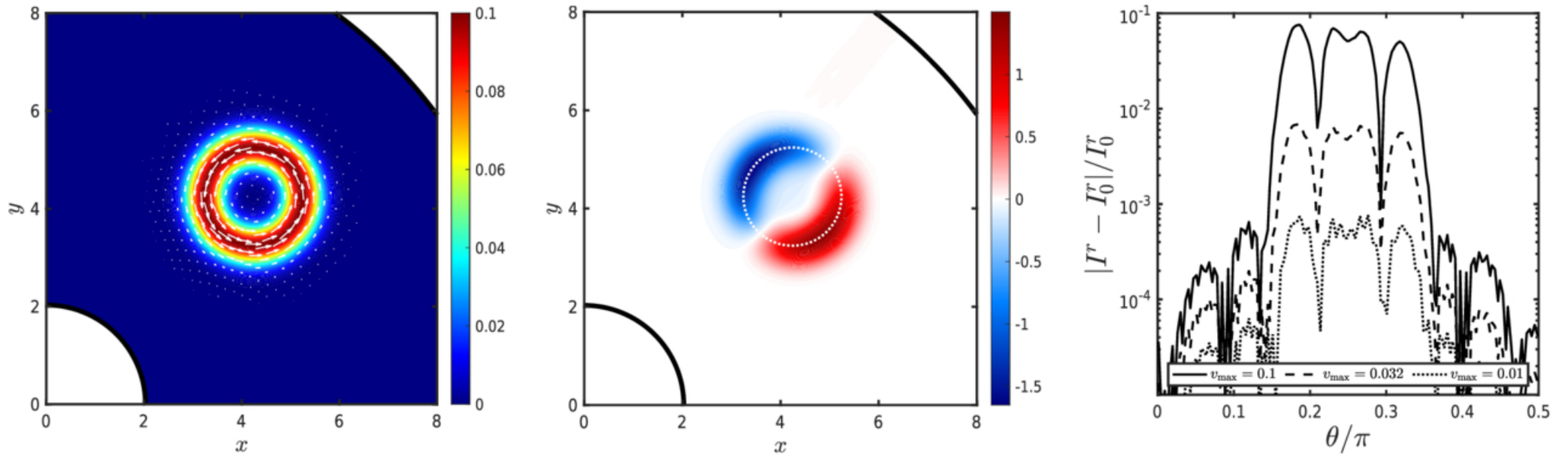
Figure 9. from Eirik Endeve et al 2026 Astrophys. J. Suppl. 284 doi:10.3847/1538-4365/ae57ad https://dx.doi.org/10.3847/1538-4365/ae57ad © 2026. The Author(s). Published by the American Astronomical Society.
