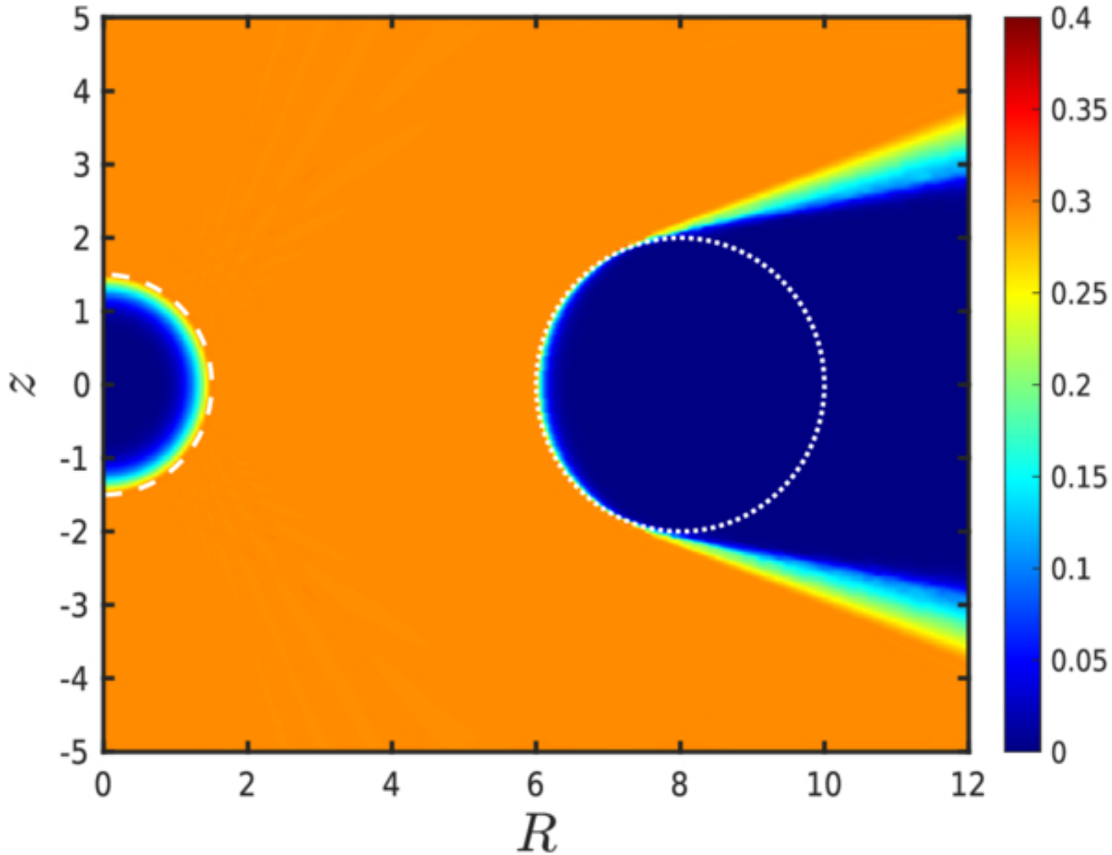
Figure 8. from Eirik Endeve et al 2026 Astrophys. J. Suppl. 284 doi:10.3847/1538-4365/ae57ad https://dx.doi.org/10.3847/1538-4365/ae57ad © 2026. The Author(s). Published by the American Astronomical Society.
