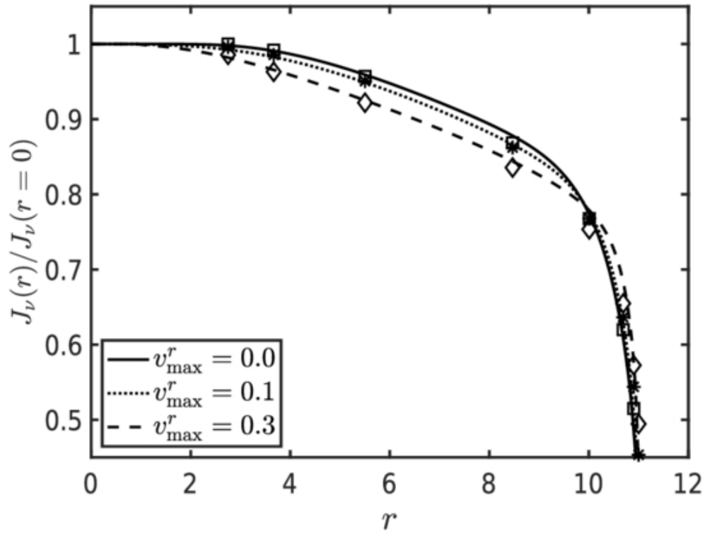
Figure 7. from Eirik Endeve et al 2026 Astrophys. J. Suppl. 284 doi:10.3847/1538-4365/ae57ad https://dx.doi.org/10.3847/1538-4365/ae57ad © 2026. The Author(s). Published by the American Astronomical Society.
