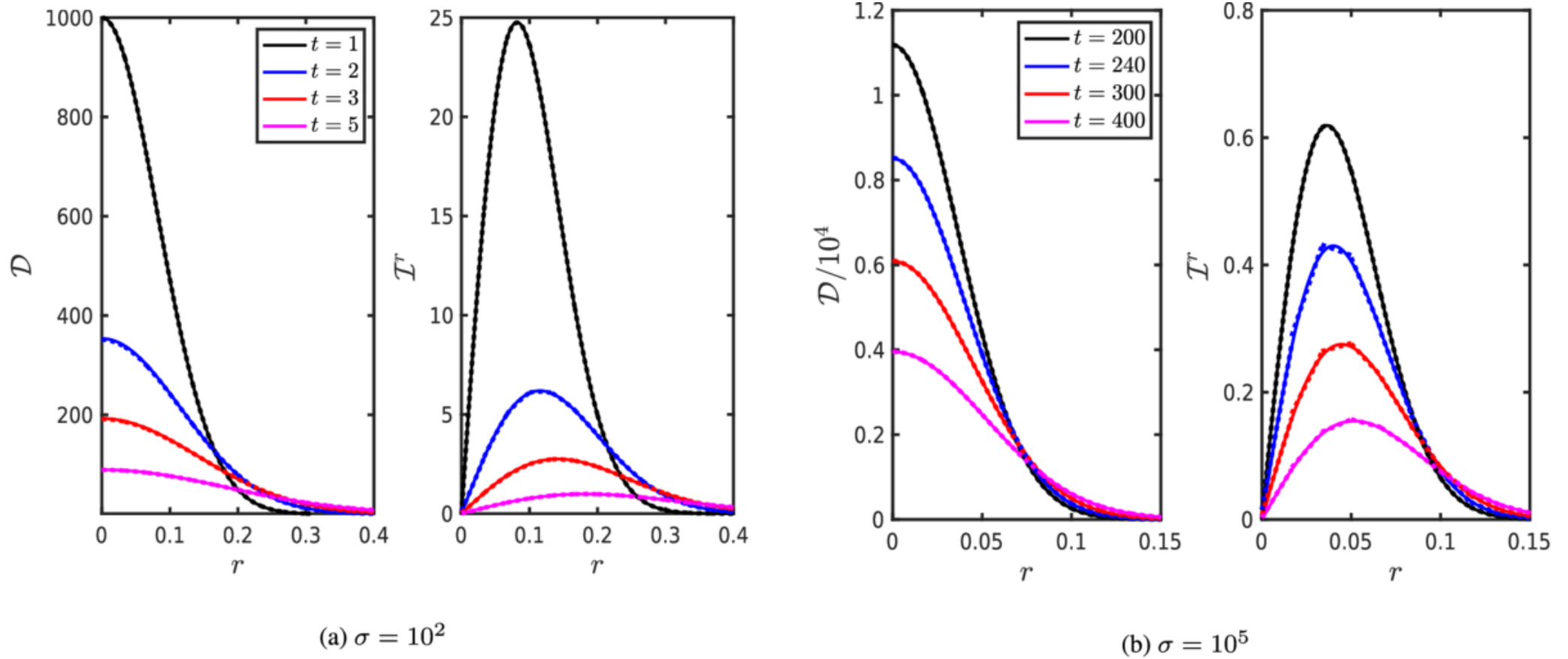
Figure 5. from Eirik Endeve et al 2026 Astrophys. J. Suppl. 284 doi:10.3847/1538-4365/ae57ad https://dx.doi.org/10.3847/1538-4365/ae57ad © 2026. The Author(s). Published by the American Astronomical Society.
