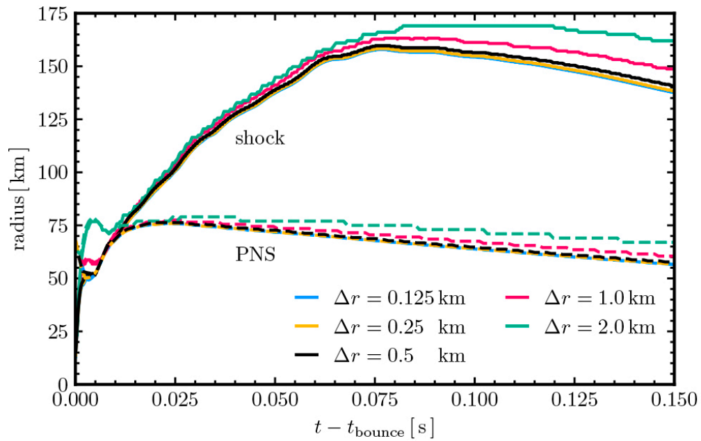
Figure 31. from Eirik Endeve et al 2026 Astrophys. J. Suppl. 284 doi:10.3847/1538-4365/ae57ad https://dx.doi.org/10.3847/1538-4365/ae57ad © 2026. The Author(s). Published by the American Astronomical Society.
