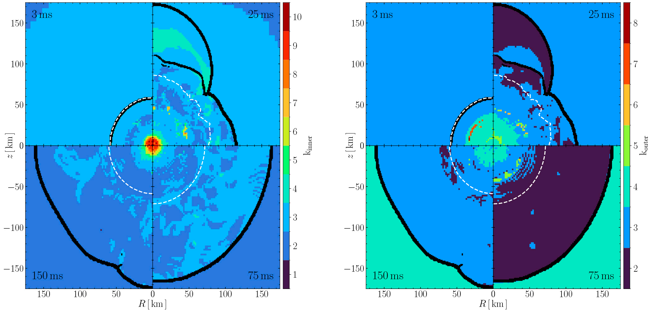
Figure 30. from Eirik Endeve et al 2026 Astrophys. J. Suppl. 284 doi:10.3847/1538-4365/ae57ad https://dx.doi.org/10.3847/1538-4365/ae57ad © 2026. The Author(s). Published by the American Astronomical Society.
