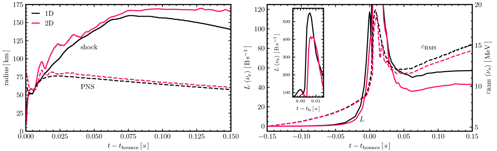
Figure 29. from Eirik Endeve et al 2026 Astrophys. J. Suppl. 284 doi:10.3847/1538-4365/ae57ad https://dx.doi.org/10.3847/1538-4365/ae57ad © 2026. The Author(s). Published by the American Astronomical Society.
