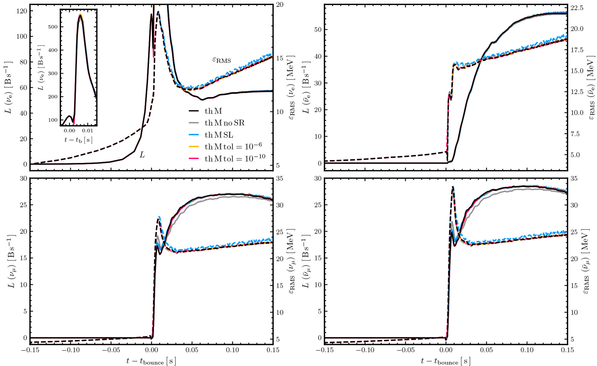
Figure 26. from Eirik Endeve et al 2026 Astrophys. J. Suppl. 284 doi:10.3847/1538-4365/ae57ad https://dx.doi.org/10.3847/1538-4365/ae57ad © 2026. The Author(s). Published by the American Astronomical Society.
