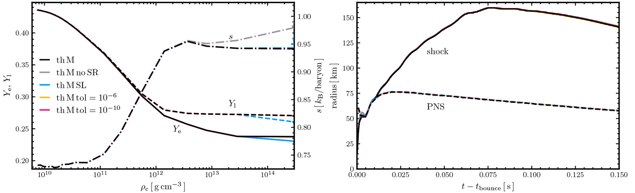
Figure 25. from Eirik Endeve et al 2026 Astrophys. J. Suppl. 284 doi:10.3847/1538-4365/ae57ad https://dx.doi.org/10.3847/1538-4365/ae57ad © 2026. The Author(s). Published by the American Astronomical Society.
