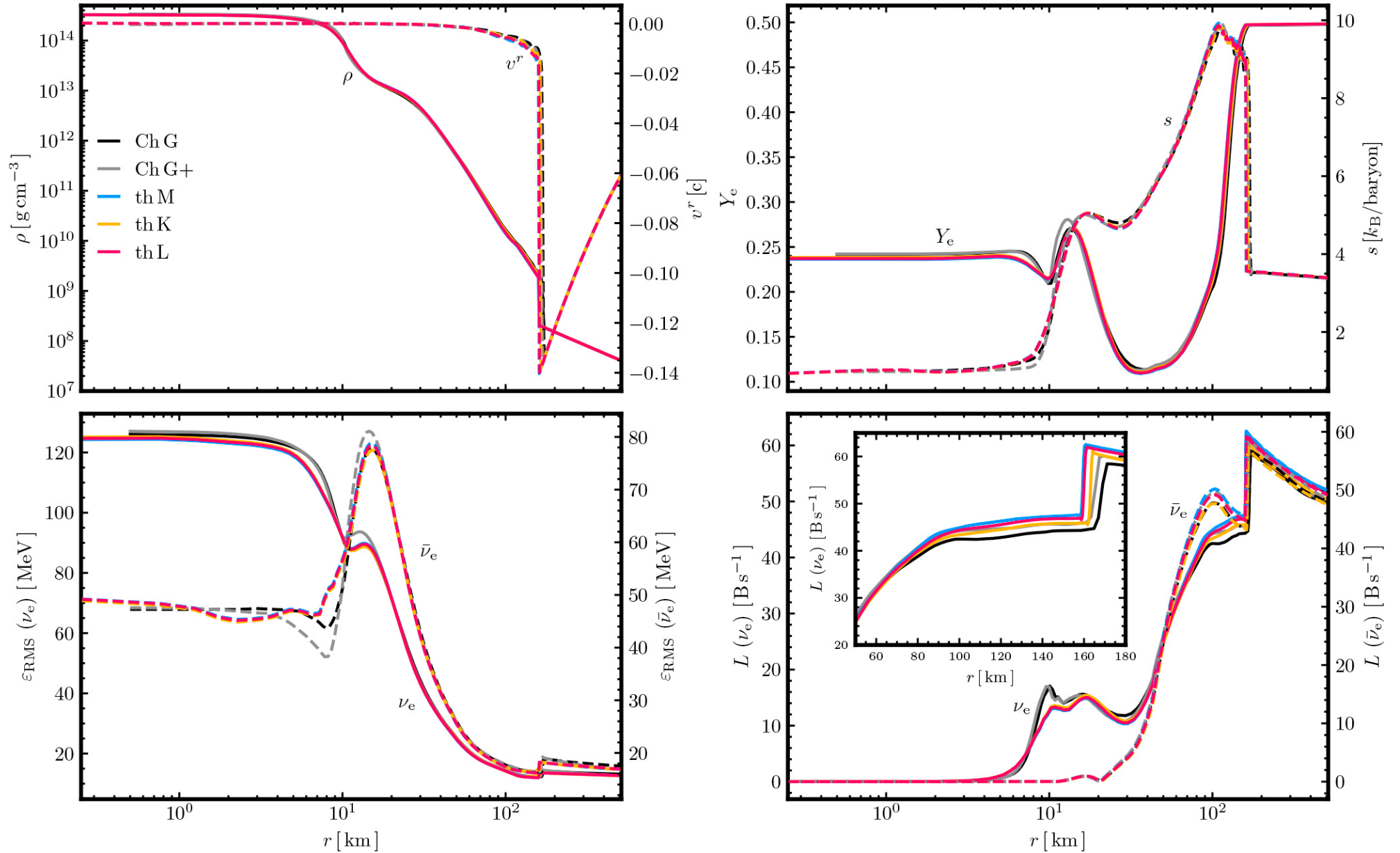
Figure 23. from Eirik Endeve et al 2026 Astrophys. J. Suppl. 284 doi:10.3847/1538-4365/ae57ad https://dx.doi.org/10.3847/1538-4365/ae57ad © 2026. The Author(s). Published by the American Astronomical Society.
