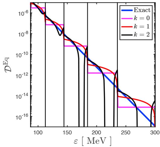
(b) Low Collisionality
