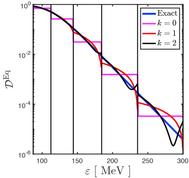
(a) High collisionality
