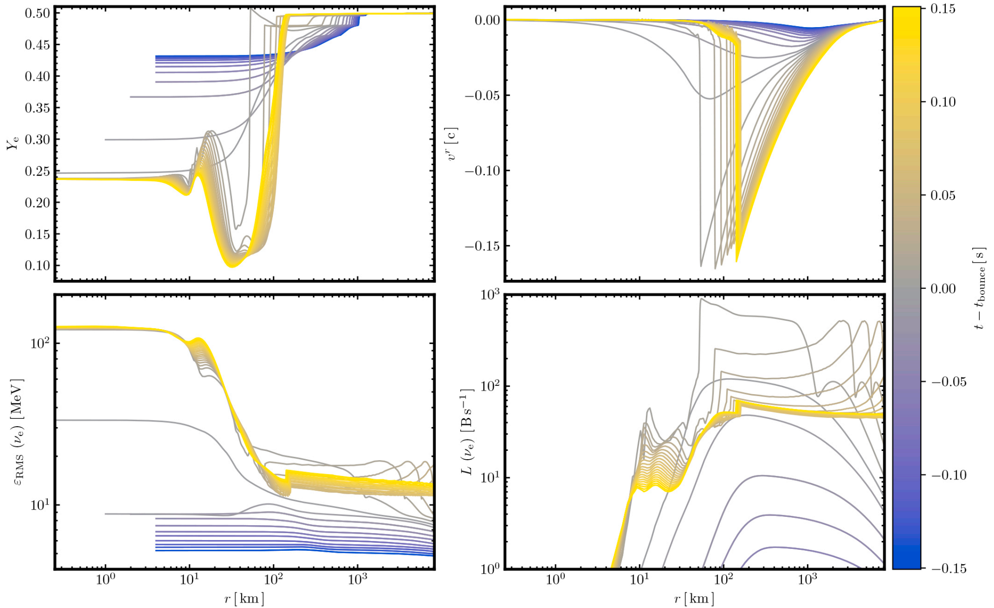
Figure 18. from Eirik Endeve et al 2026 Astrophys. J. Suppl. 284 doi:10.3847/1538-4365/ae57ad https://dx.doi.org/10.3847/1538-4365/ae57ad © 2026. The Author(s). Published by the American Astronomical Society.
