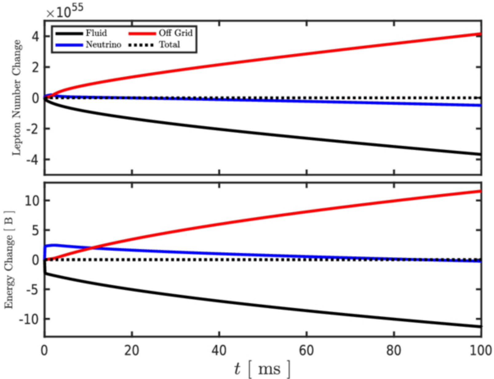
Figure 17. from Eirik Endeve et al 2026 Astrophys. J. Suppl. 284 doi:10.3847/1538-4365/ae57ad https://dx.doi.org/10.3847/1538-4365/ae57ad © 2026. The Author(s). Published by the American Astronomical Society.
